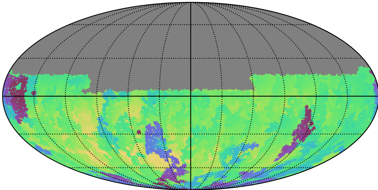
weather_cloudso31v3.4_10yrs Yr 1 u band: Min skyBrightness
