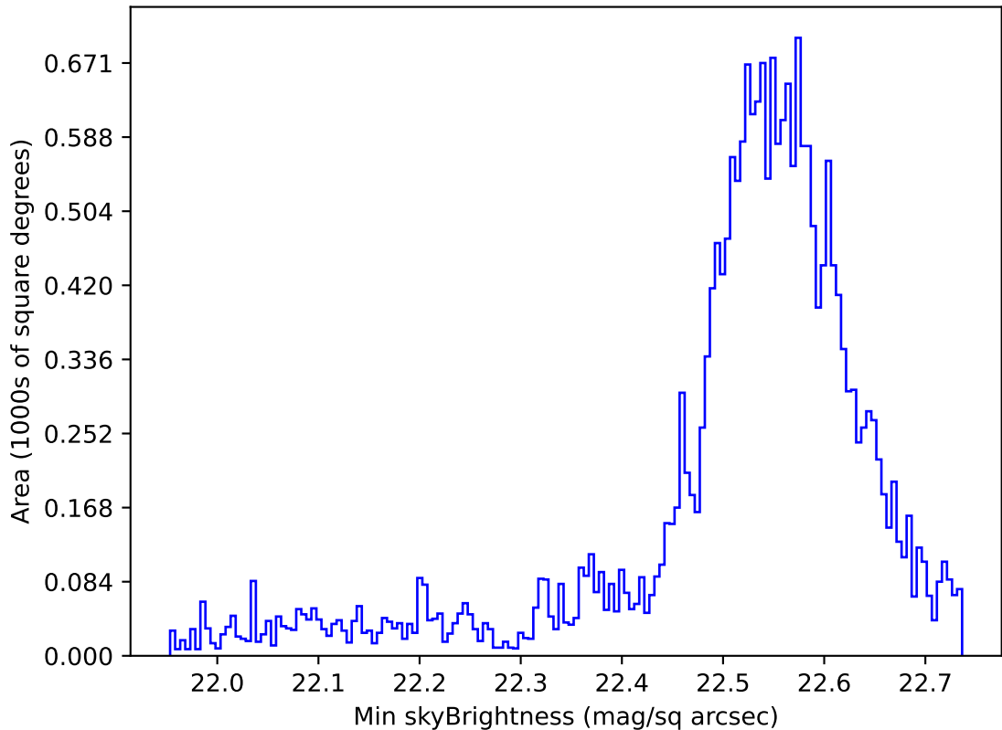
weather_cloudso31v3.4_10yrs Yr 1 u band: Min skyBrightness
