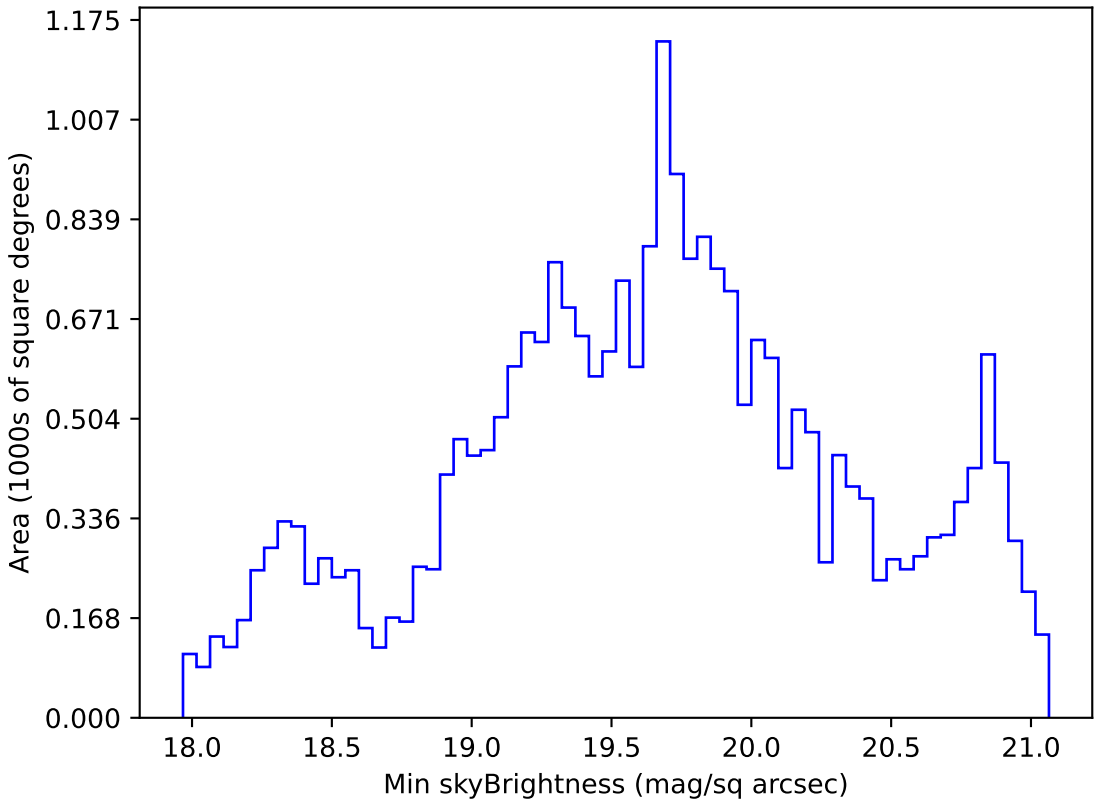
weather_cloudso31v3.4_10yrs Yr 1 r band: Min skyBrightness
