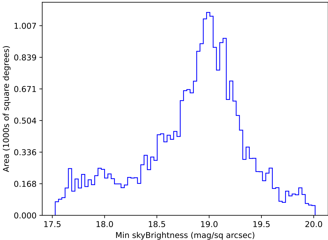
weather_cloudso31v3.4_10yrs Yr 1 i band: Min skyBrightness
