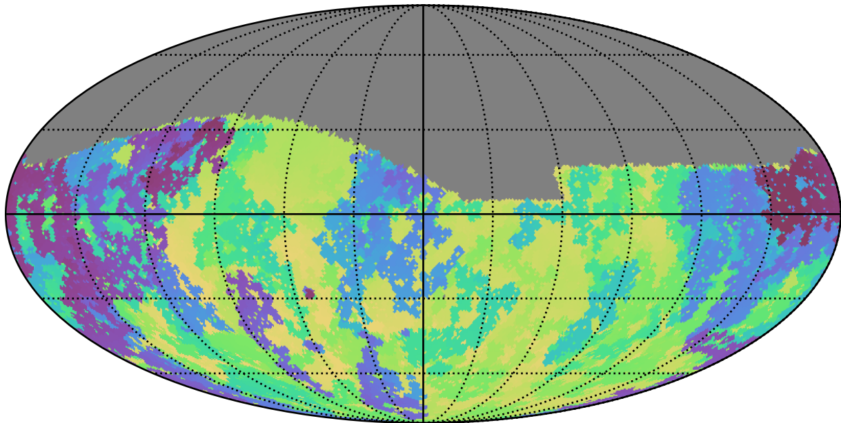
weather_cloudso31v3.4_10yrs Yr 1 g band: Min skyBrightness
