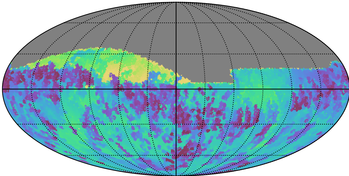
weather_cloudso31v3.4_10yrs Yr 1 all bands: Min skyBrightness
