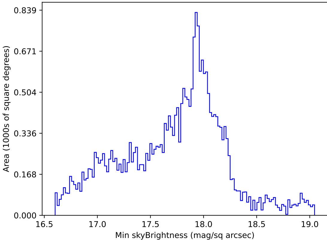
weather_cloudso31v3.4_10yrs Yr 1 all bands: Min skyBrightness
