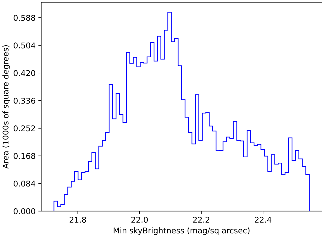
weather_cloudso31v3.4_10yrs WFD u band: Min skyBrightness
