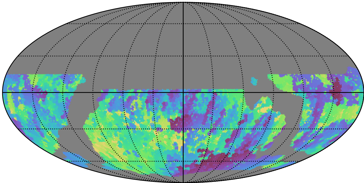
weather_cloudso31v3.4_10yrs WFD r band: Min skyBrightness
