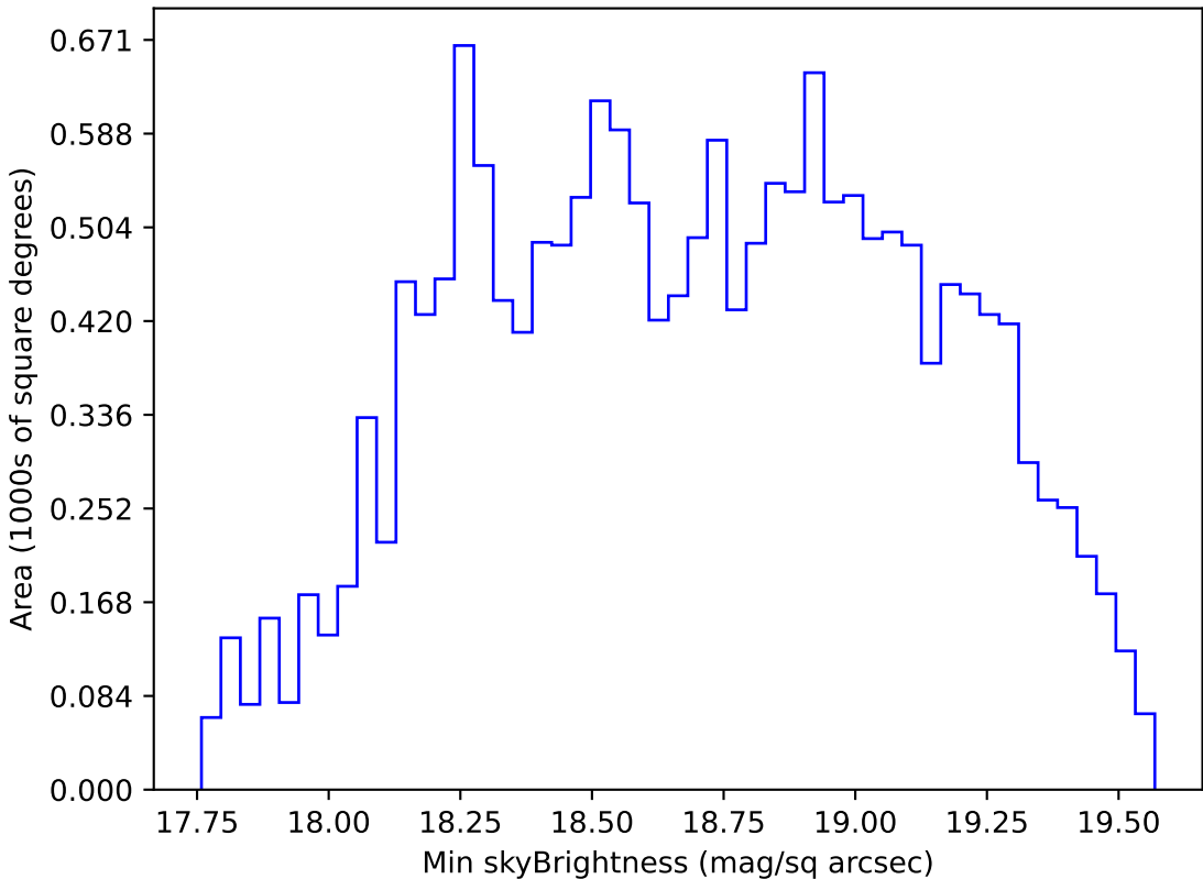
weather_cloudso31v3.4_10yrs WFD r band: Min skyBrightness
