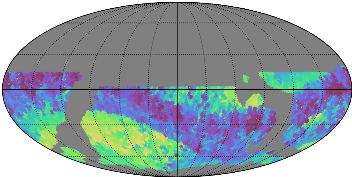
weather_cloudso31v3.4_10yrs WFD i band: Min skyBrightness
