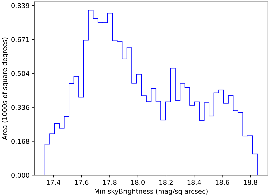
weather_cloudso31v3.4_10yrs WFD i band: Min skyBrightness
