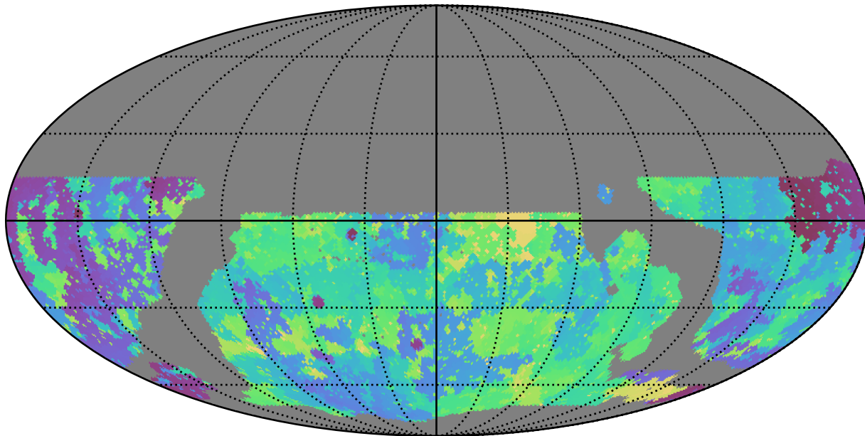
weather_cloudso31v3.4_10yrs WFD g band: Min skyBrightness
