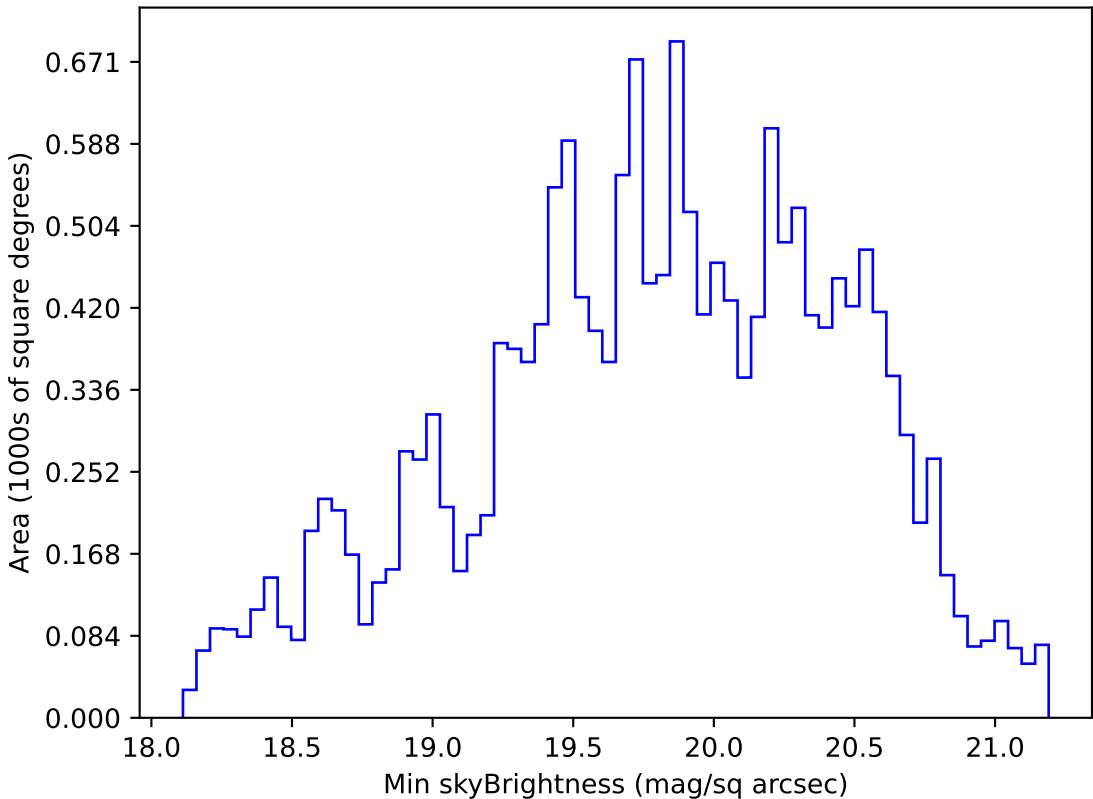
weather_cloudso31v3.4_10yrs WFD g band: Min skyBrightness
