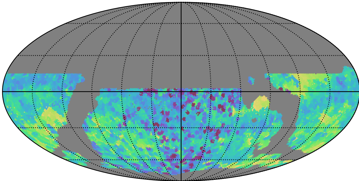
weather_cloudso31v3.4_10yrs WFD all bands: Min skyBrightness
