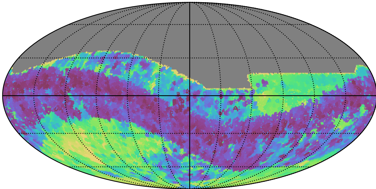
weather_cloudso31v3.4_10yrs All sky z band: Min skyBrightness
