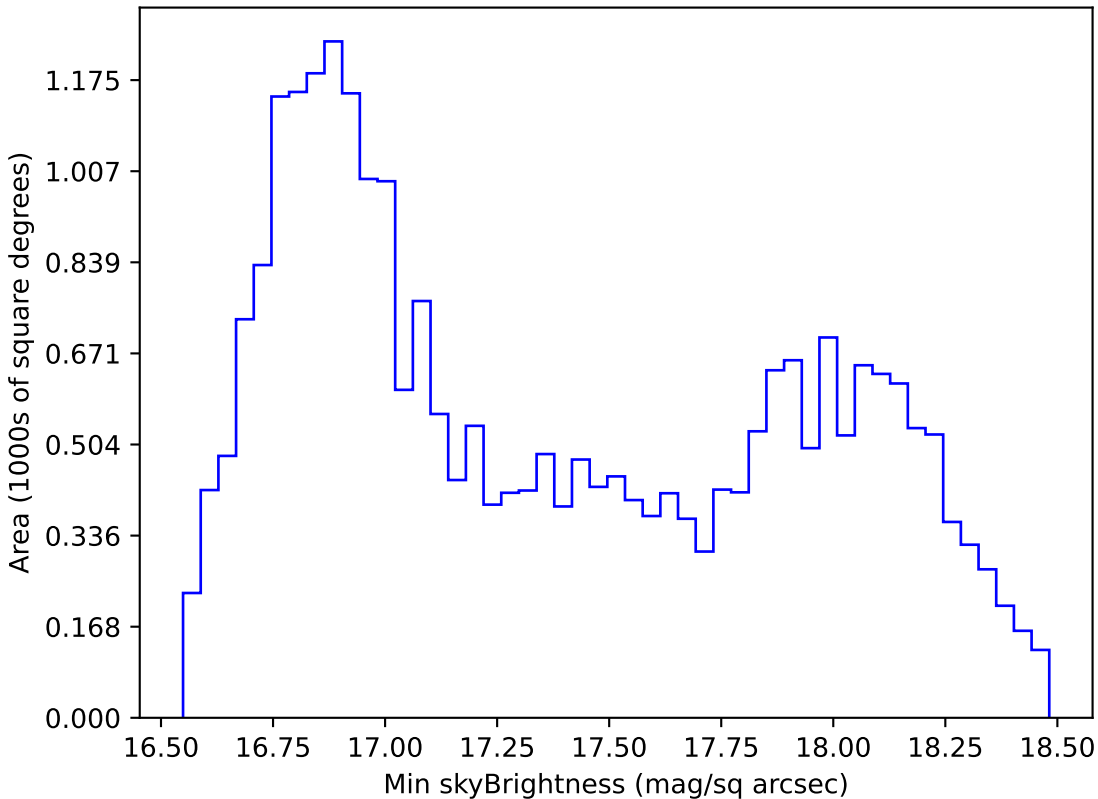
weather_cloudso31v3.4_10yrs All sky z band: Min skyBrightness
