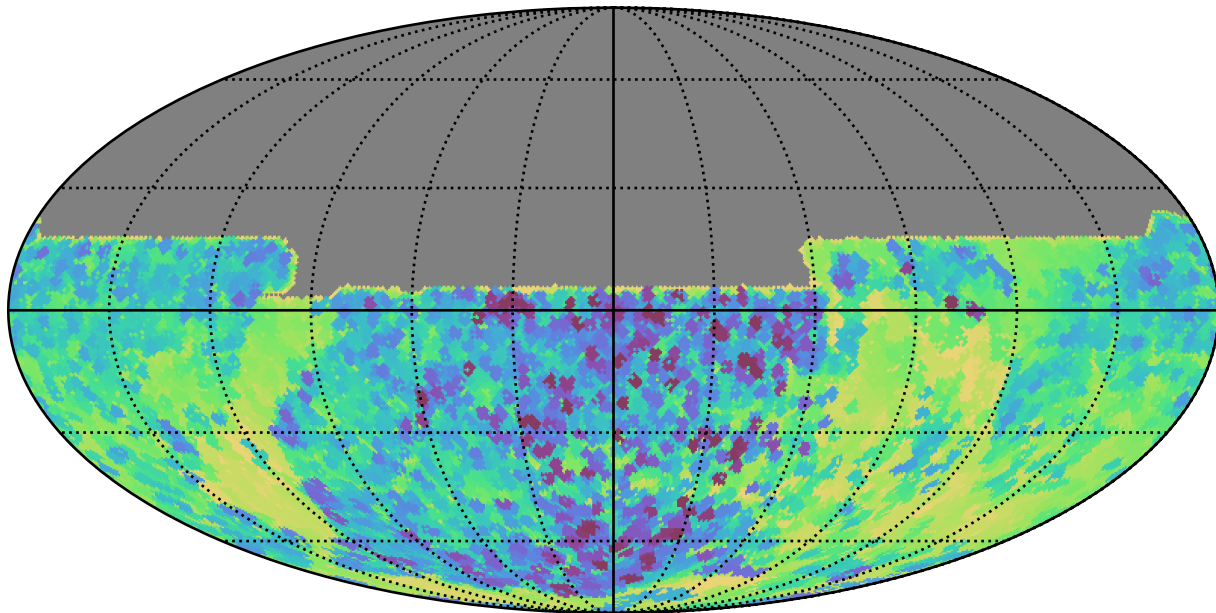
weather_cloudso31v3.4_10yrs All sky y band: Min skyBrightness
