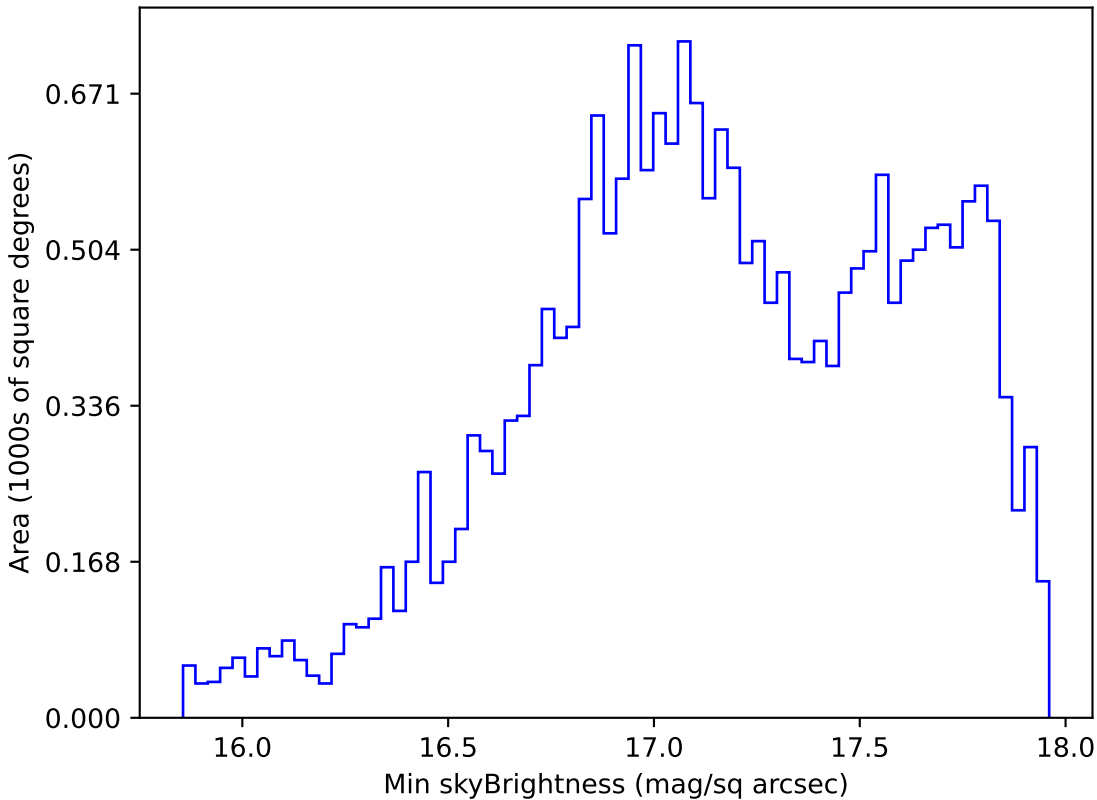
weather_cloudso31v3.4_10yrs All sky y band: Min skyBrightness
