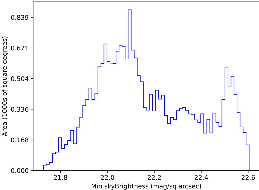
weather_cloudso31v3.4_10yrs All sky u band: Min skyBrightness
