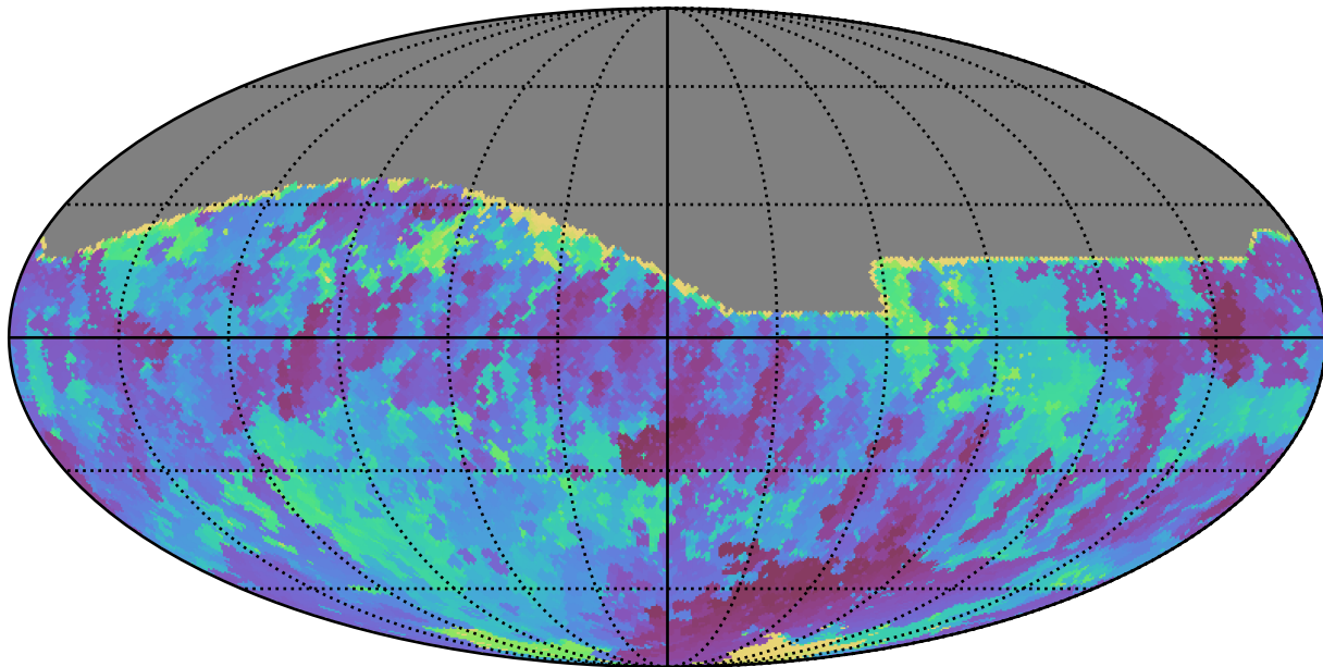
weather_cloudso31v3.4_10yrs All sky r band: Min skyBrightness
