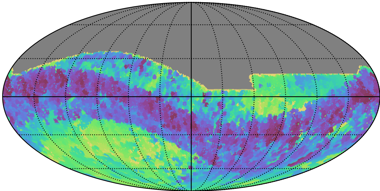
weather_cloudso31v3.4_10yrs All sky i band: Min skyBrightness
