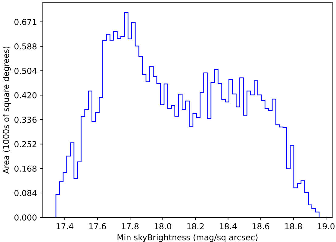
weather_cloudso31v3.4_10yrs All sky i band: Min skyBrightness
