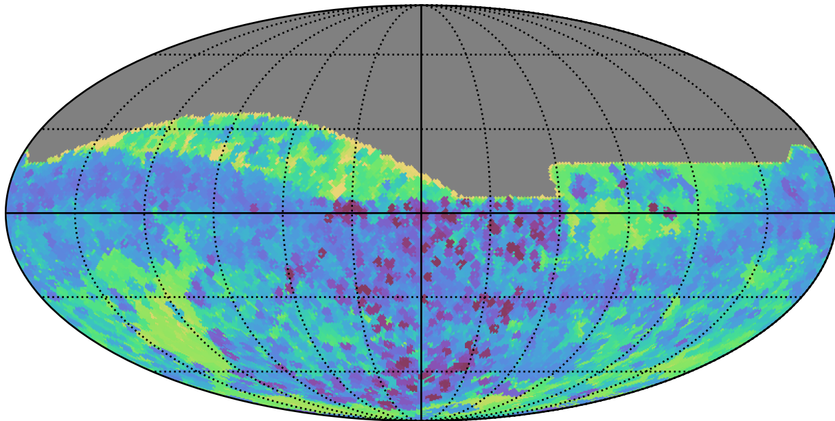
weather_cloudso31v3.4_10yrs All sky all bands: Min skyBrightness
