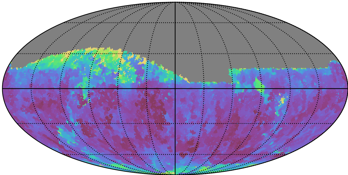
weather_cloudso31v3.4_10yrs Yr 1 z band: Min seeingGeom
