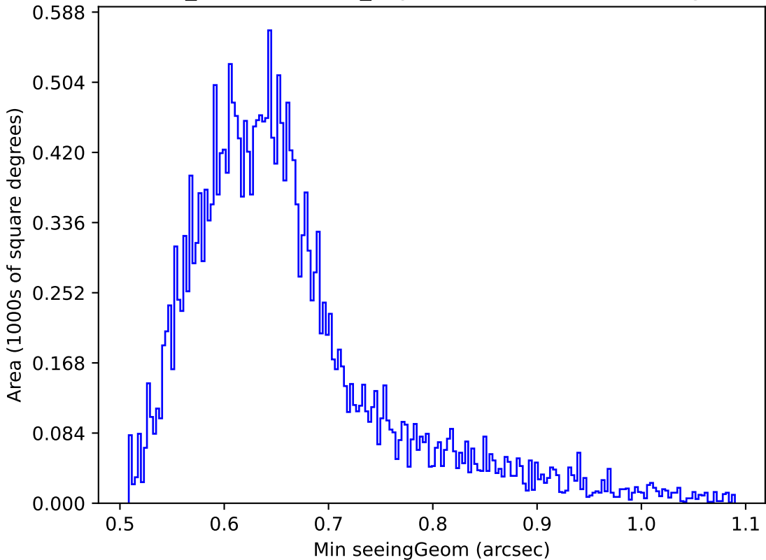
weather_cloudso31v3.4_10yrs Yr 1 z band: Min seeingGeom
