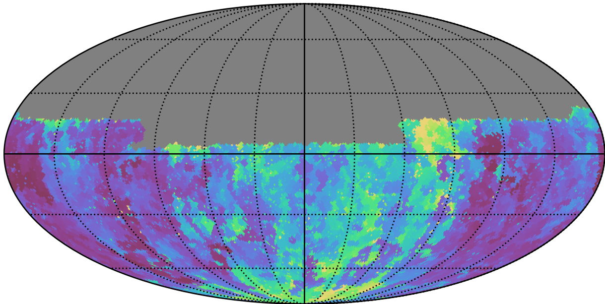
weather_cloudso31v3.4_10yrs Yr 1 u band: Min seeingGeom
