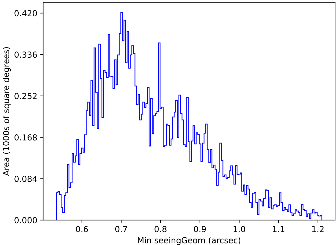
weather_cloudso31v3.4_10yrs Yr 1 u band: Min seeingGeom
