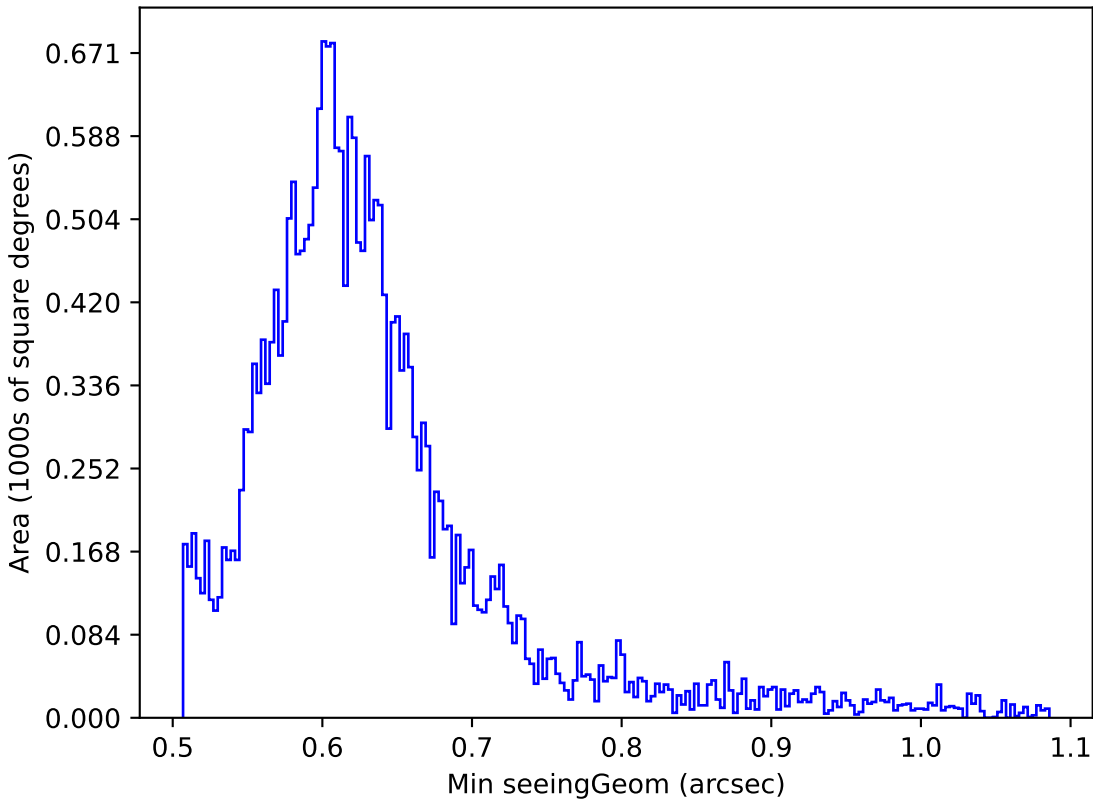
weather_cloudso31v3.4_10yrs Yr 1 r band: Min seeingGeom
