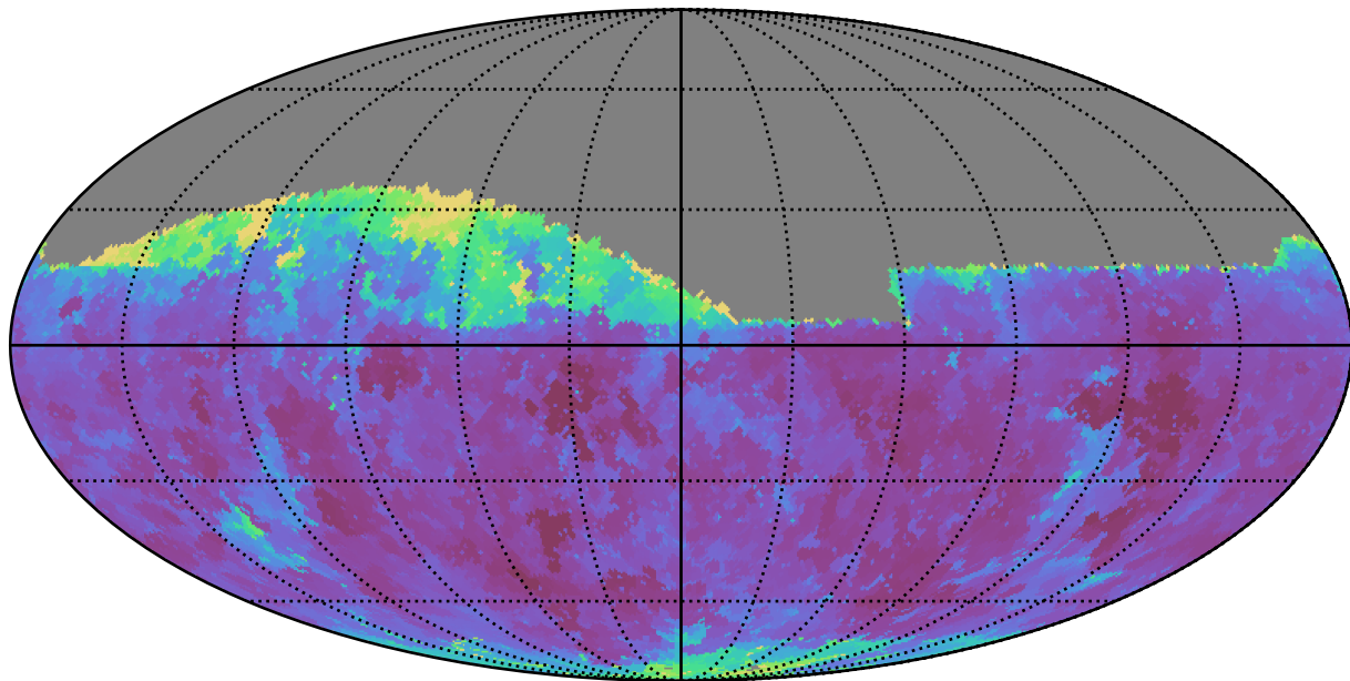
weather_cloudso31v3.4_10yrs Yr 1 i band: Min seeingGeom
