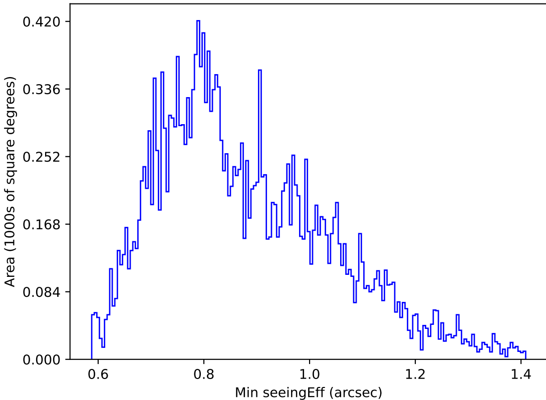
weather_cloudso31v3.4_10yrs Yr 1 u band: Min seeingEff
