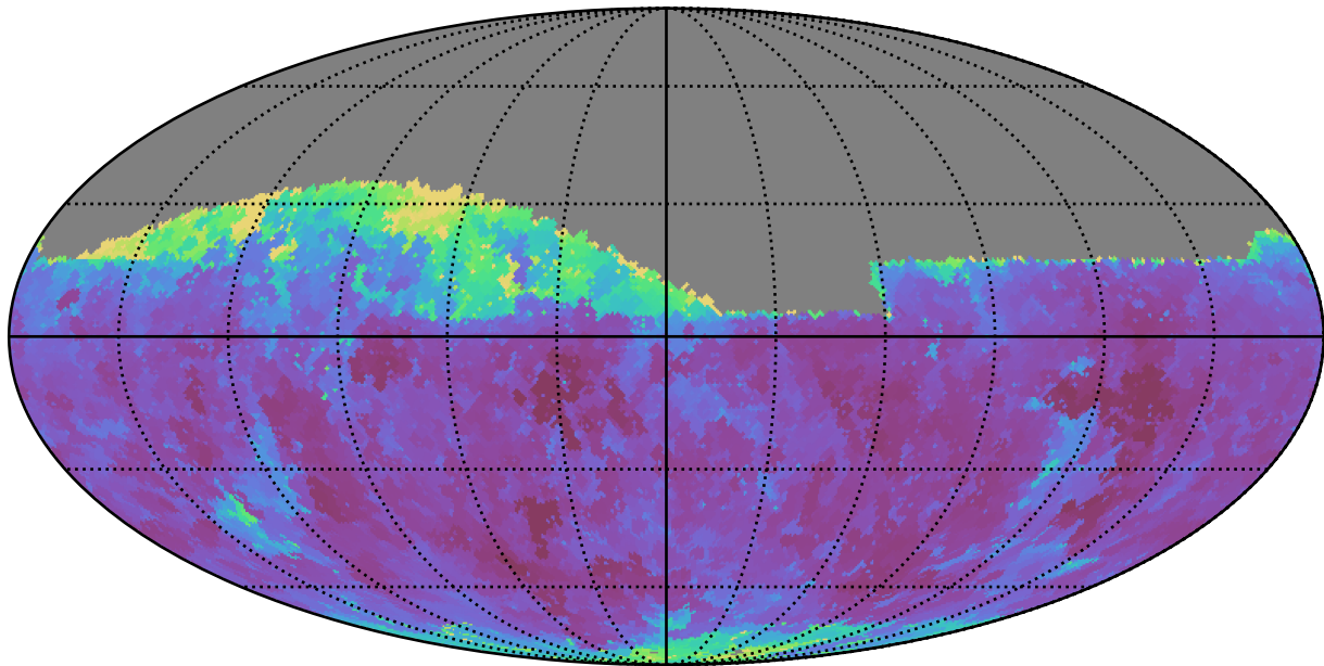
weather_cloudso31v3.4_10yrs Yr 1 i band: Min seeingEff
