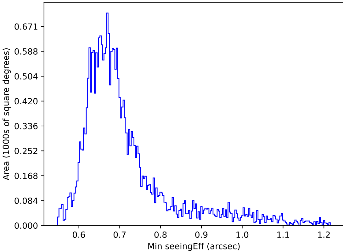
weather_cloudso31v3.4_10yrs Yr 1 i band: Min seeingEff
