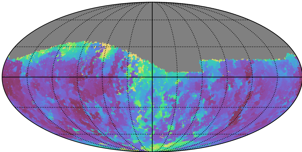
weather_cloudso31v3.4_10yrs Yr 1 g band: Min seeingEff
