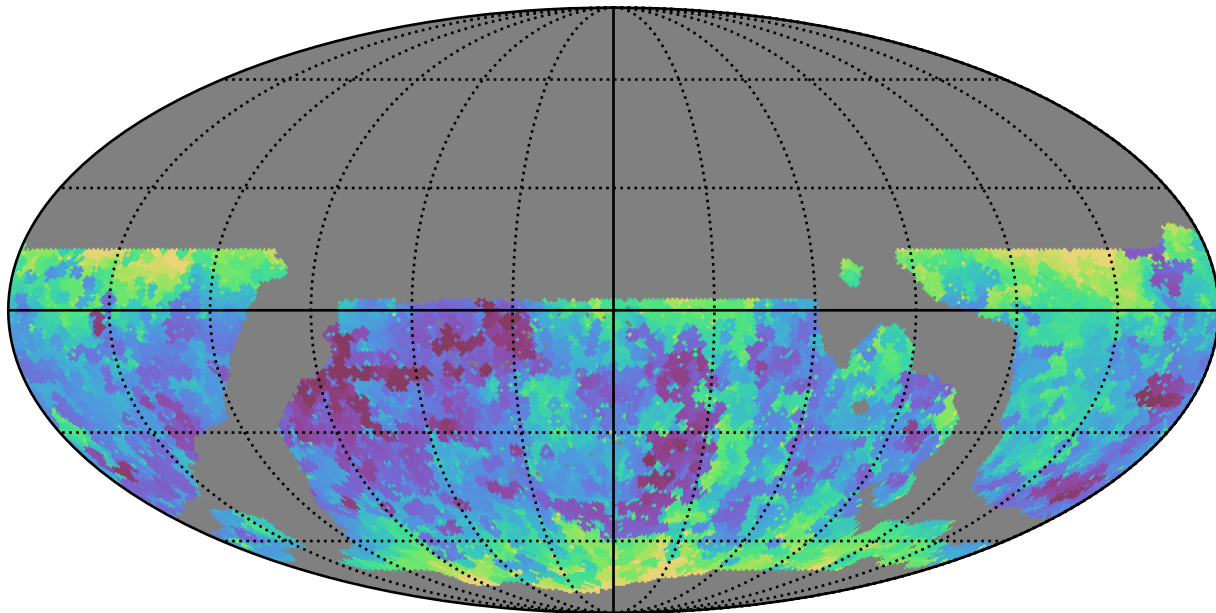
weather_cloudso31v3.4_10yrs WFD y band: Min seeingEff
