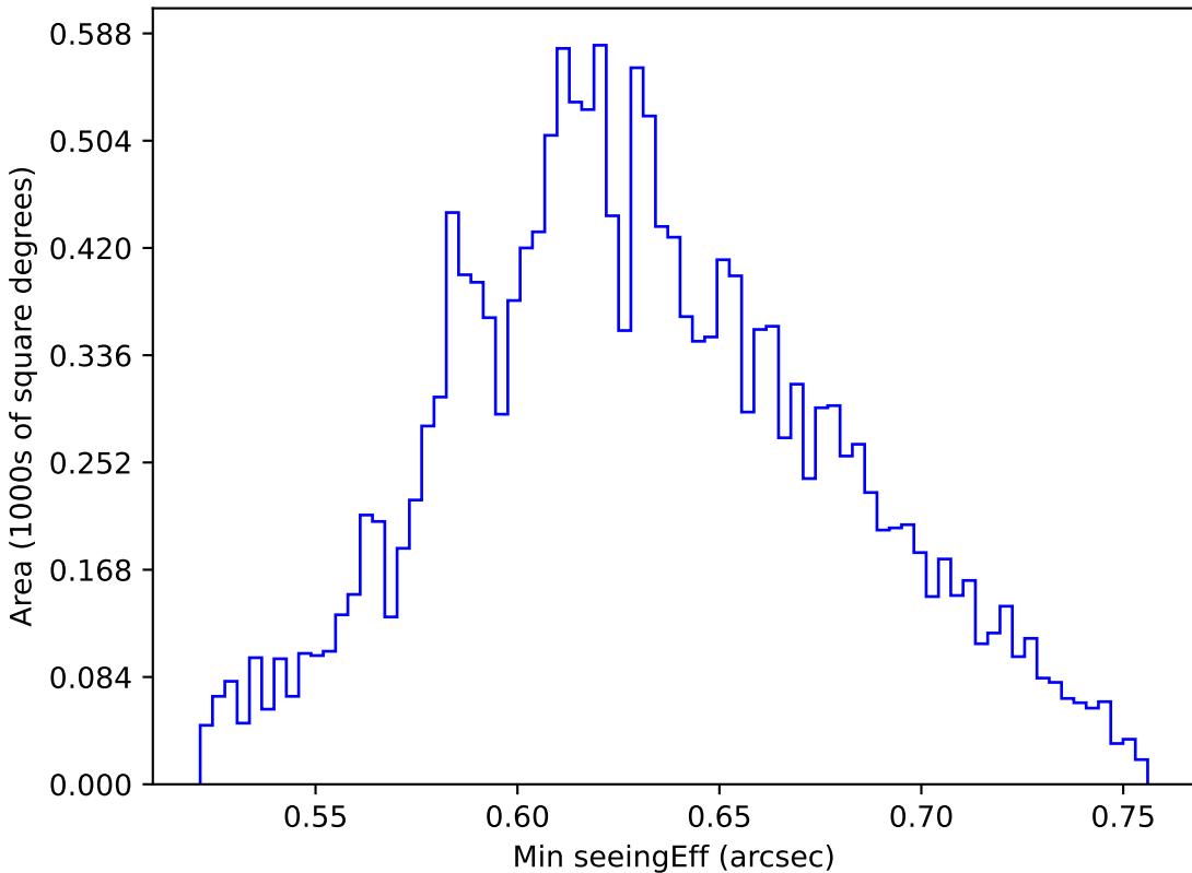
weather_cloudso31v3.4_10yrs WFD y band: Min seeingEff
