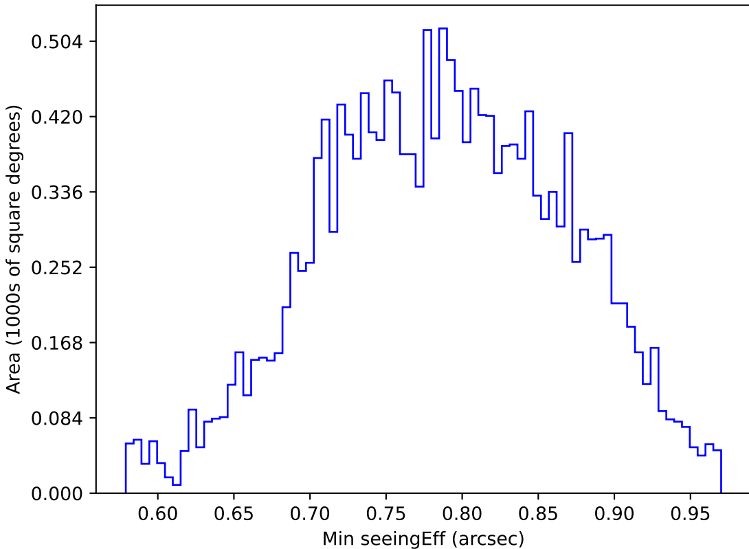
weather_cloudso31v3.4_10yrs WFD u band: Min seeingEff
