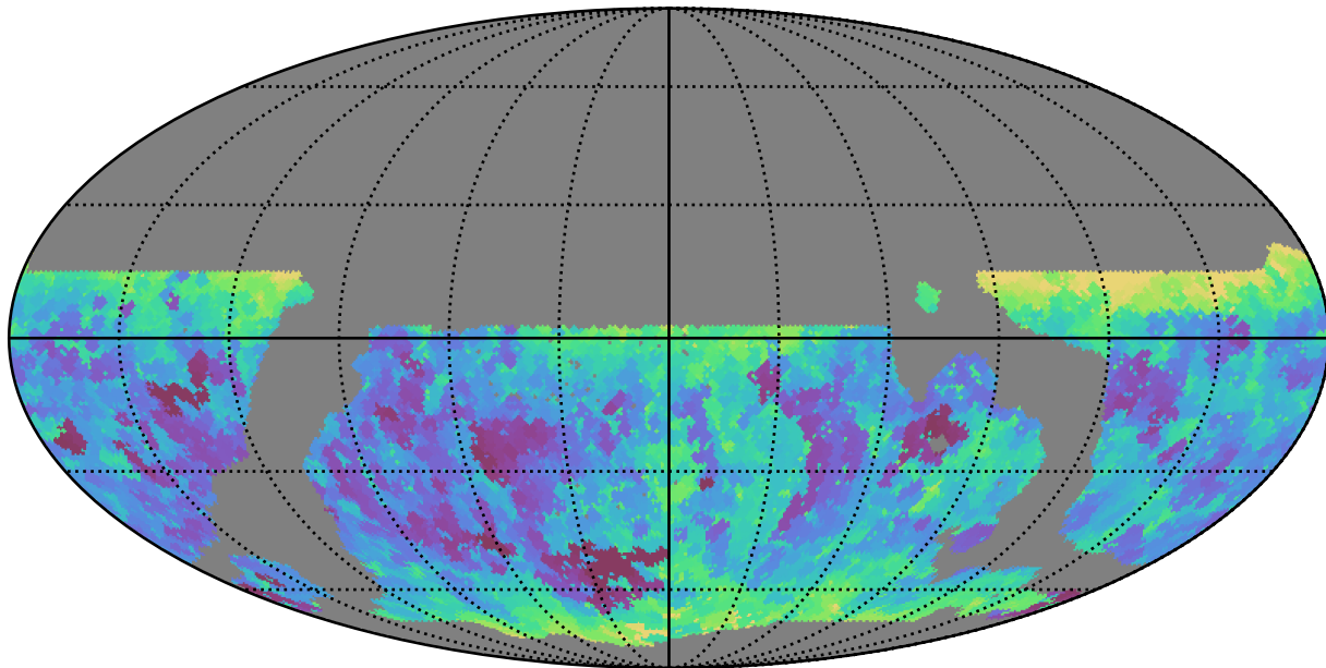
weather_cloudso31v3.4_10yrs WFD r band: Min seeingEff
