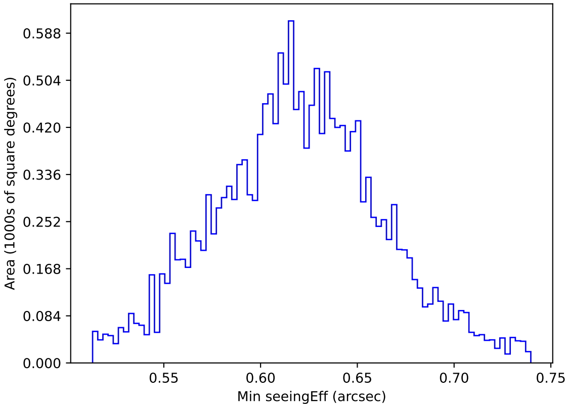
weather_cloudso31v3.4_10yrs WFD r band: Min seeingEff
