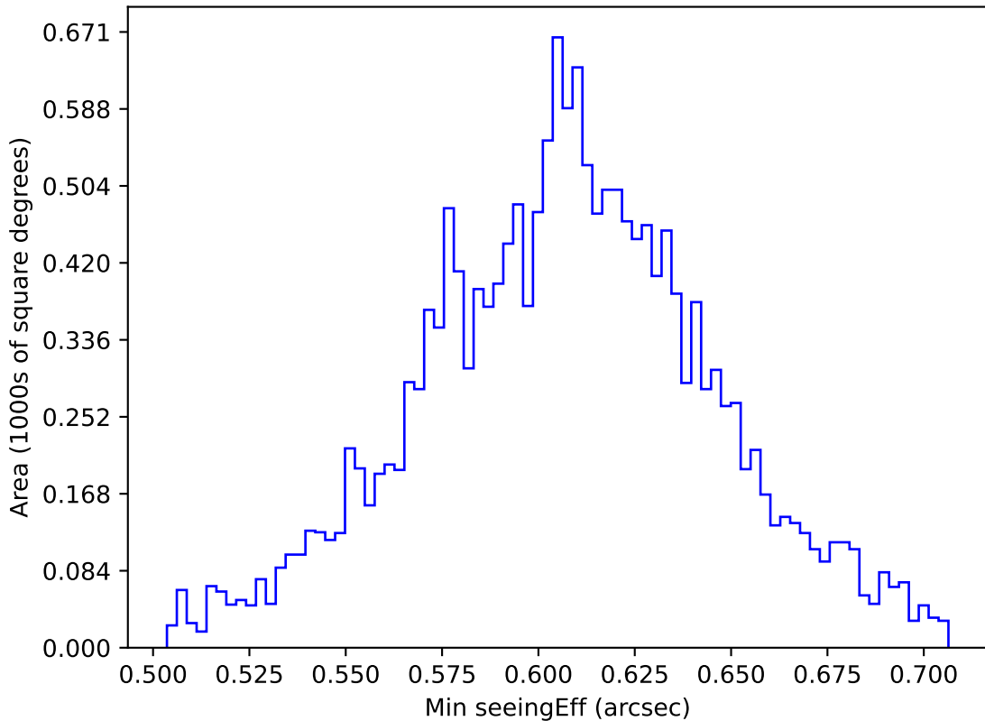
weather_cloudso31v3.4_10yrs WFD i band: Min seeingEff
