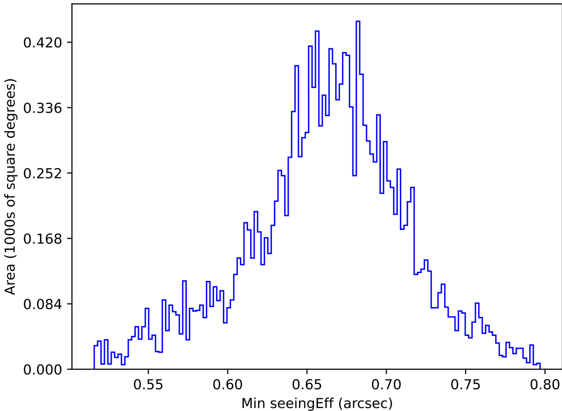
weather_cloudso31v3.4_10yrs WFD g band: Min seeingEff
