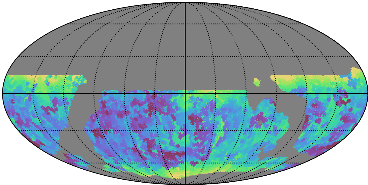
weather_cloudso31v3.4_10yrs WFD all bands: Min seeingEff
