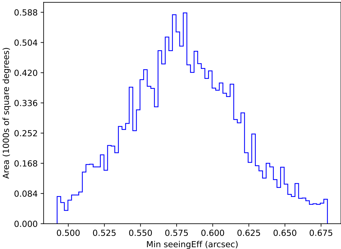
weather_cloudso31v3.4_10yrs WFD all bands: Min seeingEff
