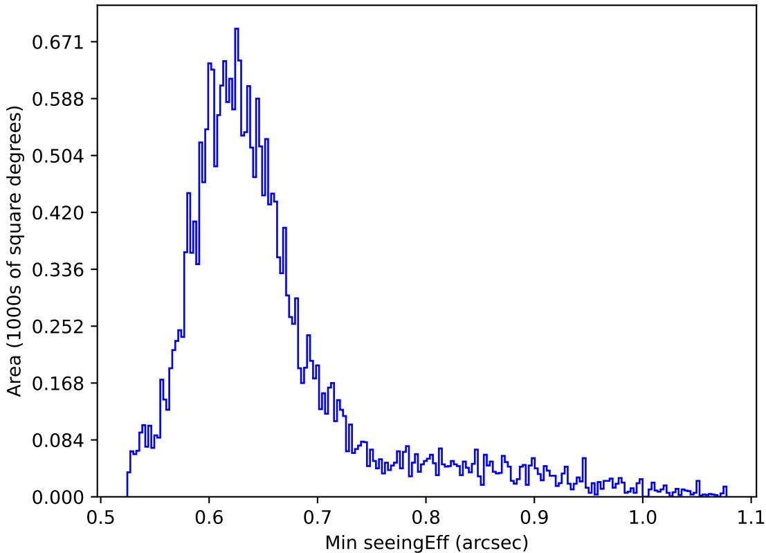
weather_cloudso31v3.4_10yrs All sky z band: Min seeingEff
