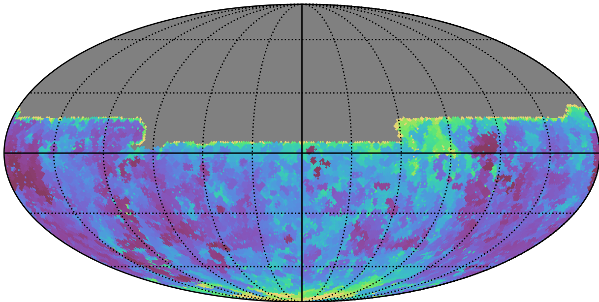
weather_cloudso31v3.4_10yrs All sky u band: Min seeingEff
