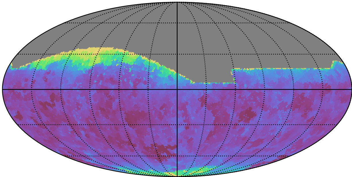
weather_cloudso31v3.4_10yrs All sky r band: Min seeingEff
