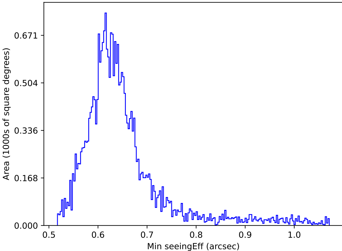
weather_cloudso31v3.4_10yrs All sky r band: Min seeingEff
