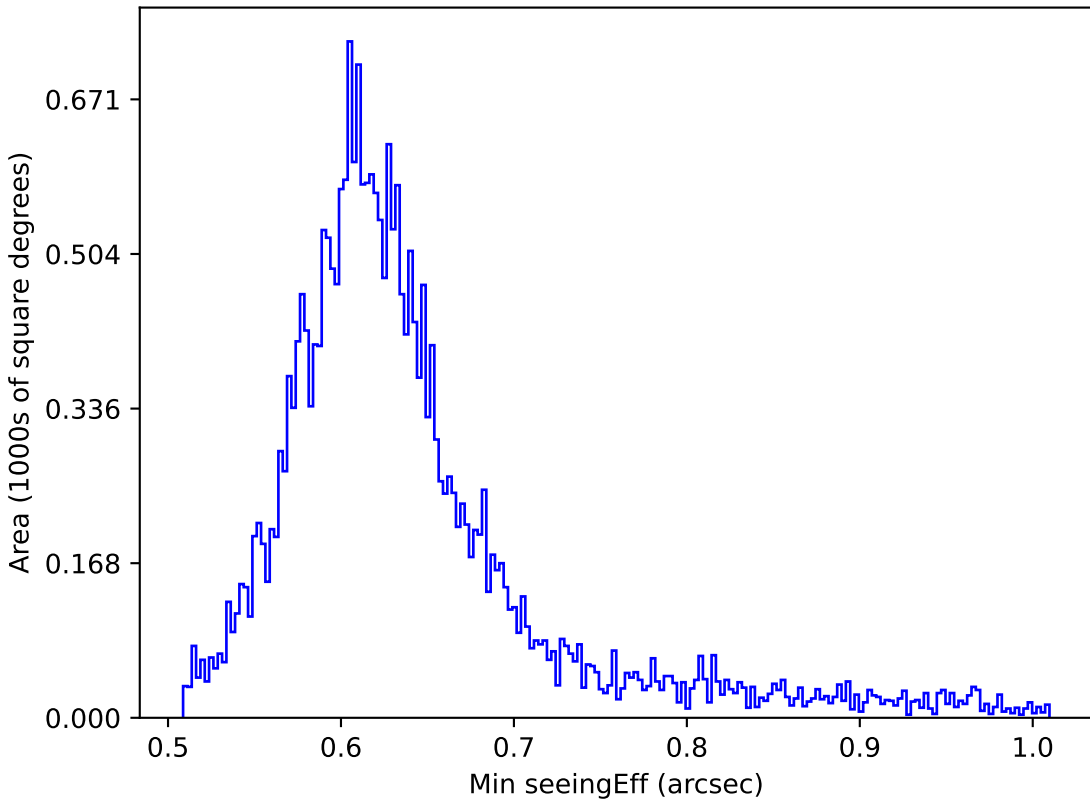
weather_cloudso31v3.4_10yrs All sky i band: Min seeingEff
