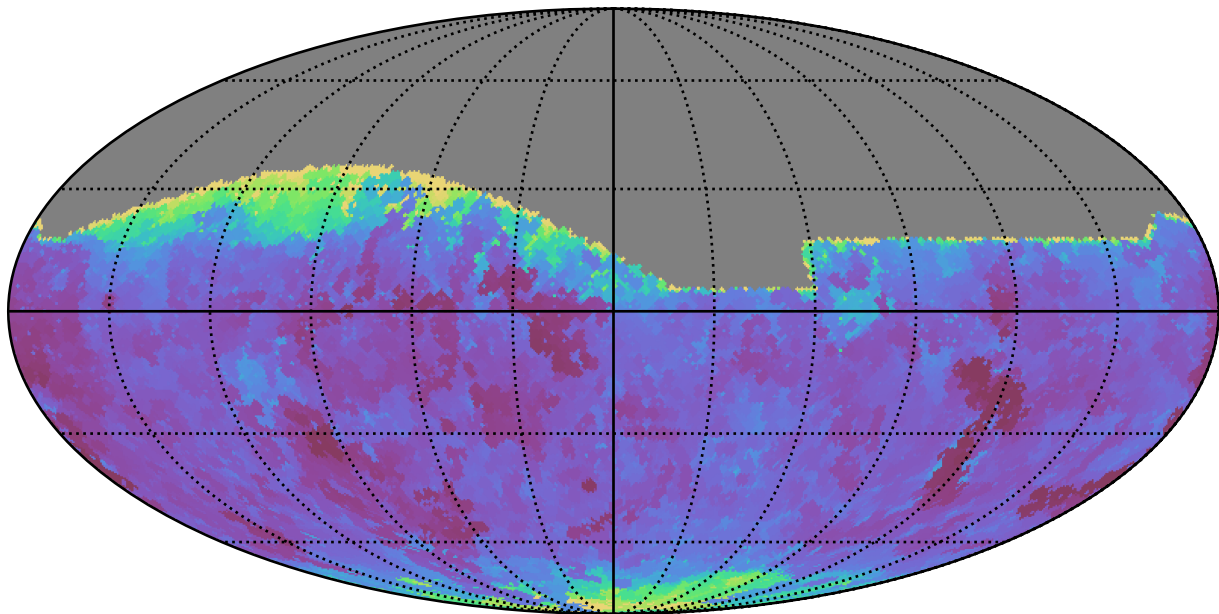
weather_cloudso31v3.4_10yrs All sky g band: Min seeingEff
