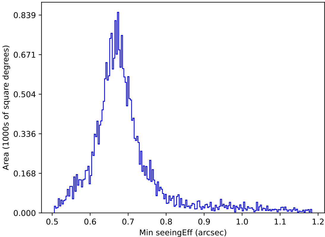
weather_cloudso31v3.4_10yrs All sky g band: Min seeingEff
